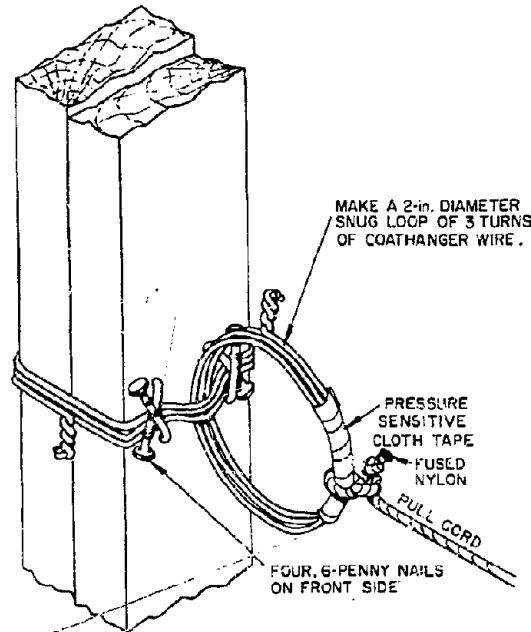
Fig. B-20. Connection of pull-cord to center brace.
